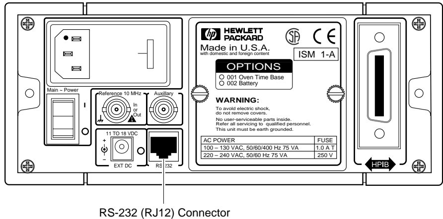
Figure 3-2. Location of the RS-232 (RJ12) Connector
