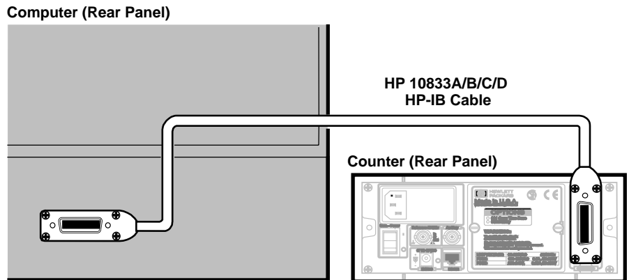
Figure 3-1. HP-IB Interconnection
